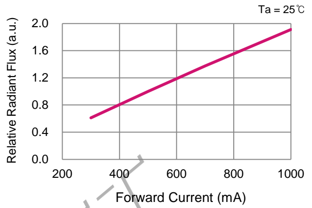
■ Forward Current vs. Relative Radiant Flux
